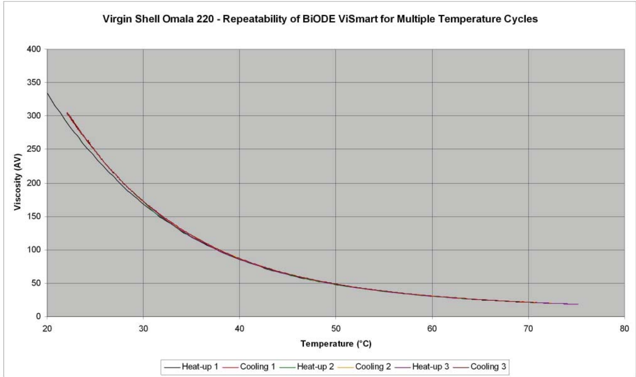
Figure 3: Repeatability of viscosity data using the ViSmart
