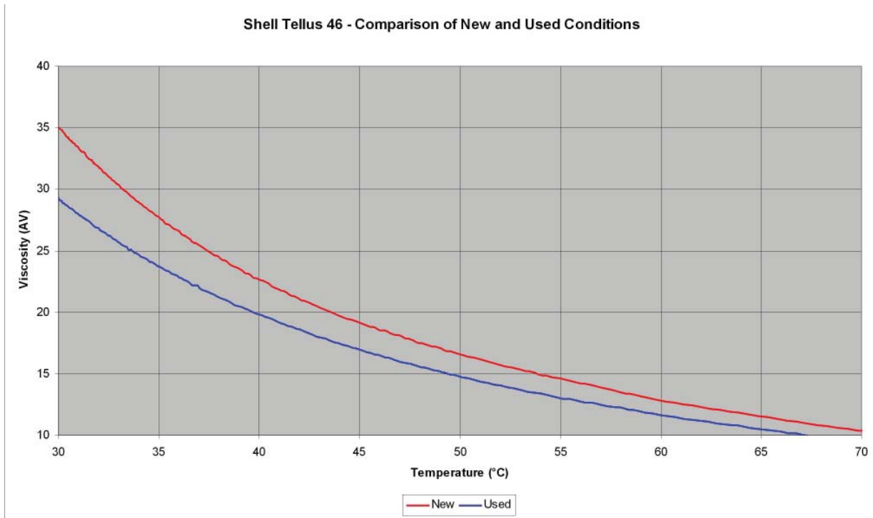
Figure 1: Monitoring of oil condition as a function of use and temperature using the Vismart
