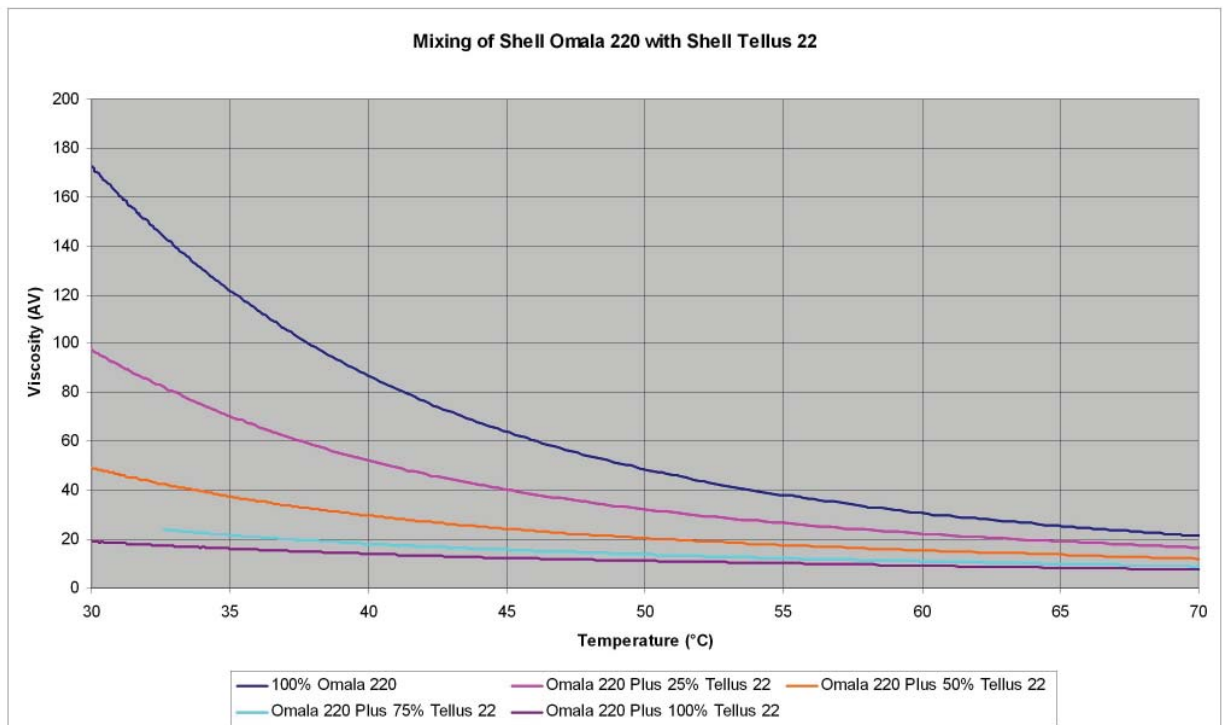
Figure 2: Monitoring the viscosity of two different grades of oil using the ViSmart
